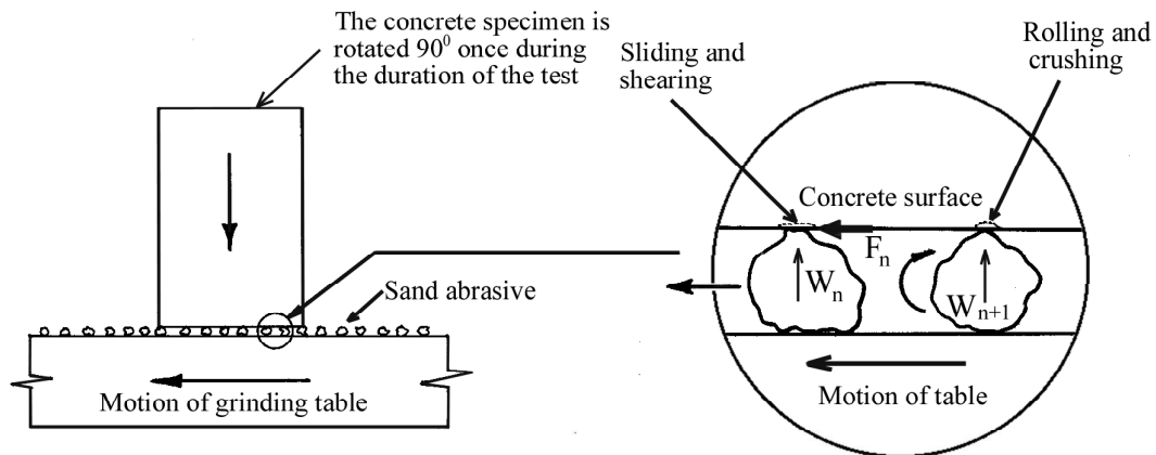
Figure U.5.5.3 Rolling and sliding wear mechanisms
