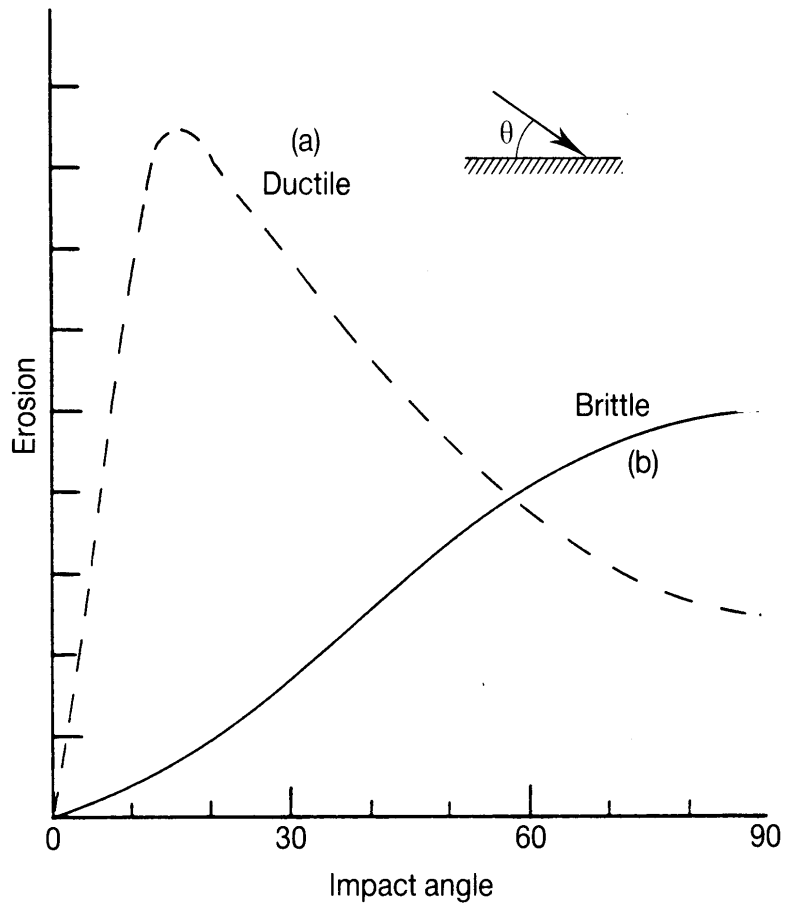
Figure 4.3 Influence of angle of attack on abrasion wear. [Hutchings(1992)].
