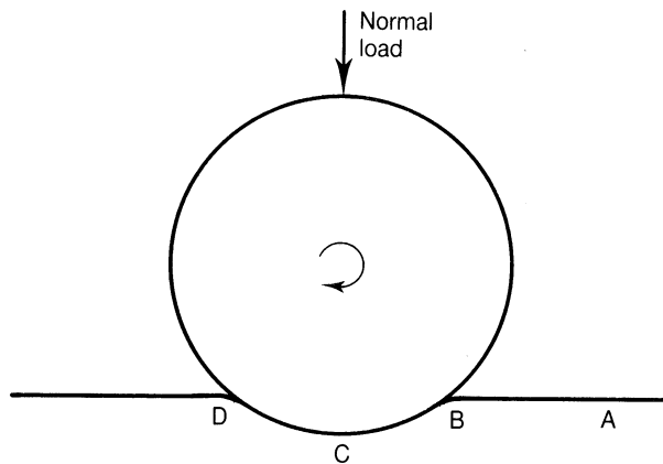
Figure 4.1 Cross section through a sphere or cylinder rolling over an elastic surface, illustrating the origin of Reynolds slip. [Hutchings(1992)].
