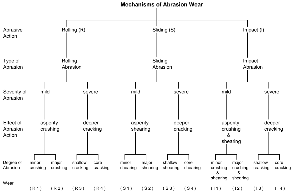
Figure 4.5 Elements that make up the abrasion wear code
