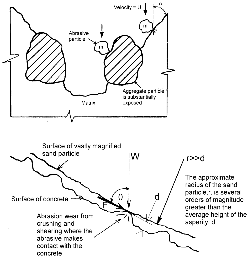
Figure 4.4 (a) The abrasive sand is seen to impact against the surface at an angle \theta , causing microscopic crushing and shearing effects of the surface asperities, as seen in (b).
